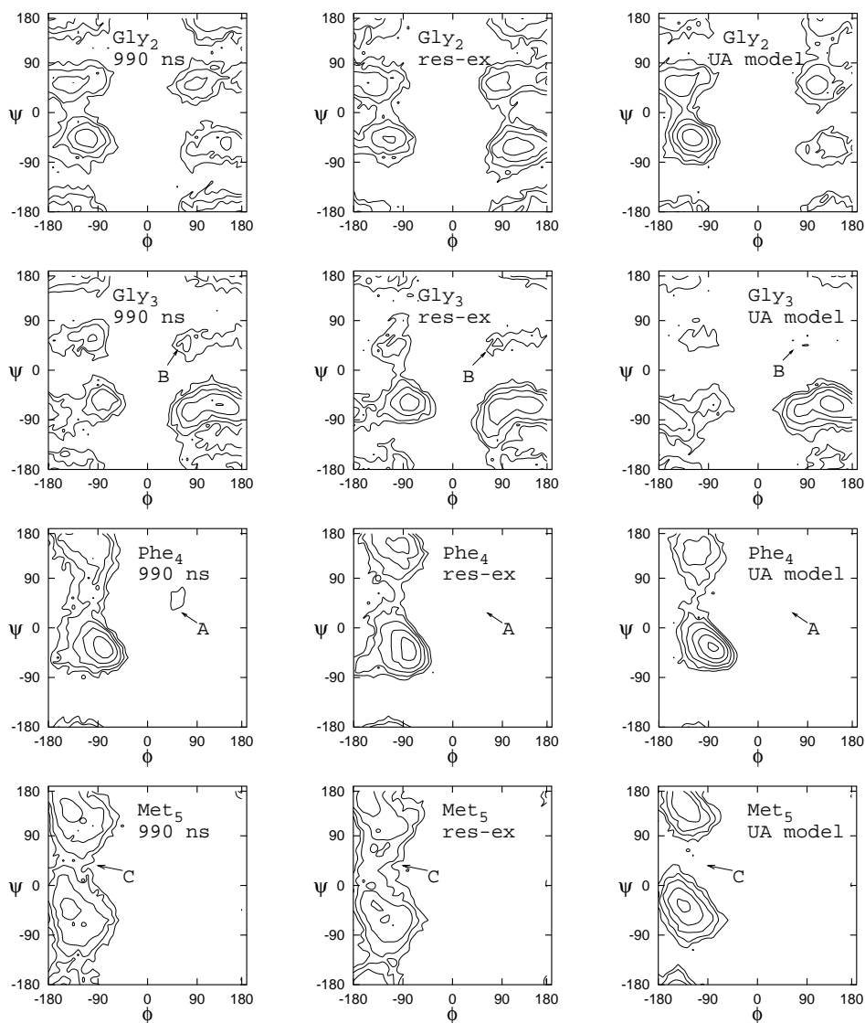
Figure 5: Ramachandran histograms for met-enkephalin. The left column is a 990 nsec Langevin dynamics simulation at all-atom resolution, without resolution exchange; the middle column is the all-atom level ( M_0 ) from resolution exchange as described in the text; the right column is the top-level united-atom simulation (level M_5 ) used for the resolution exchange simulation shown in the middle column. Note that since the peptide is unblocked, there are only 4 pairs of \phi - \psi dihedrals. Res-ex fails to “find” one region (labelled “A”) not present in the top-level simulation, but finds two others (labelled “B” and “C”).
