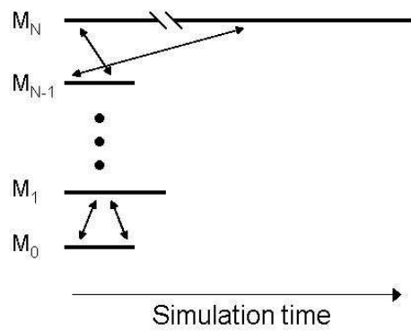
Figure 2: Schematic representation of top-down exchange. Thick horizontal lines are simulation trajectories (labelled “ M_i ” for model “ i ”) and arrows represent exchanges. The M_i may differ in resolution, temperature, or both. Notice that the top level simulation may be considerably longer than the others.
